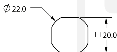
CUT-OUT
