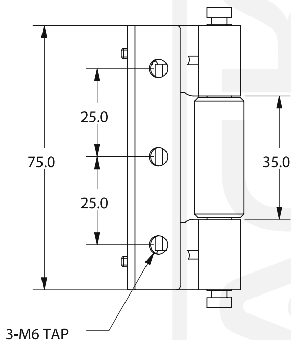
SHEET METAL HINGE
