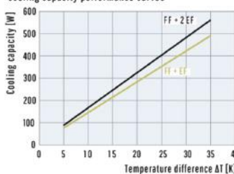
Cooling capacity performance curves
